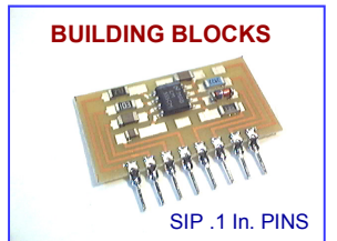
Many SURFBOARDS feature SIP (single-in-line) pins on .1 inch centers for compatibility with both traditional and solderless breadboards and sockets. Just add parts and plug in.
